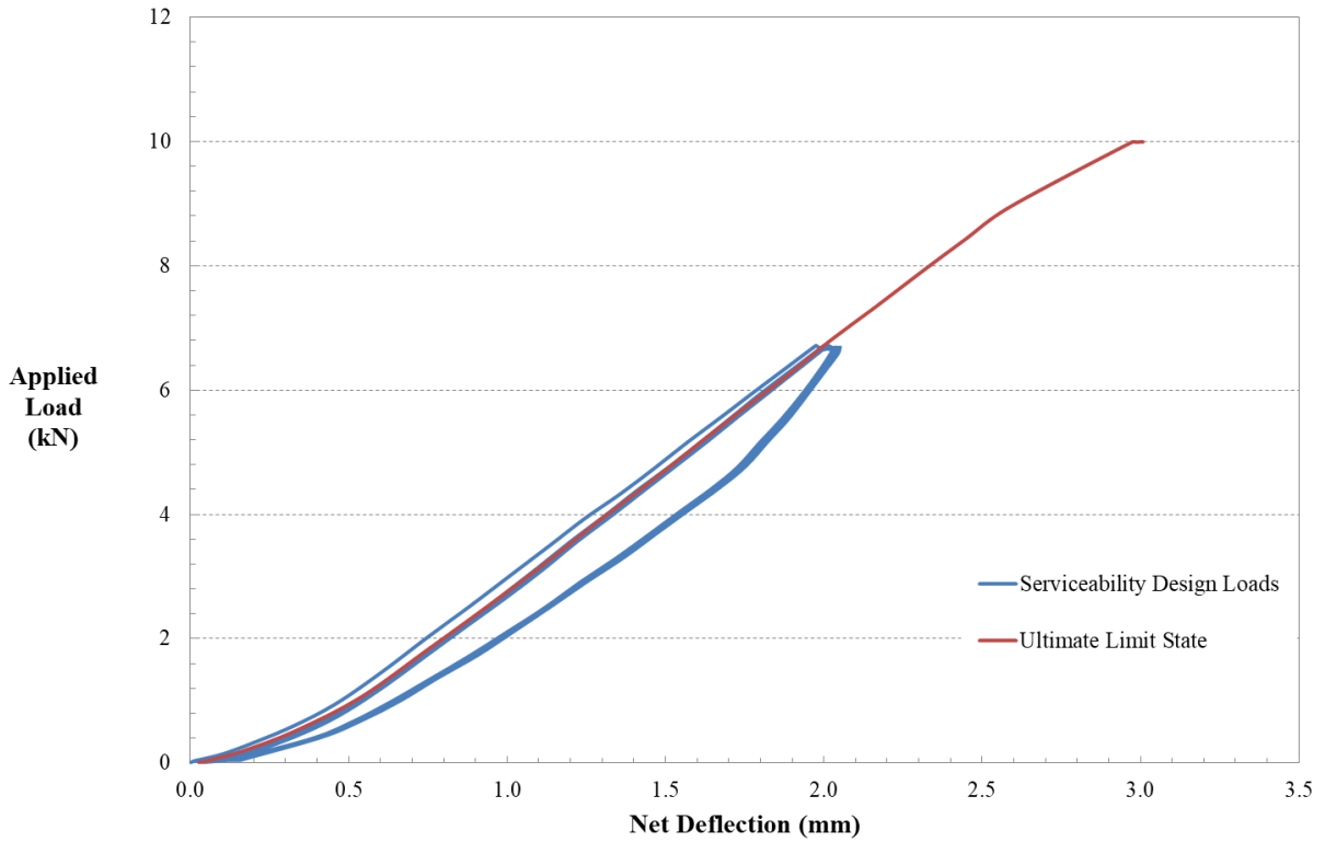
FIG. 3 TEST CURVES
