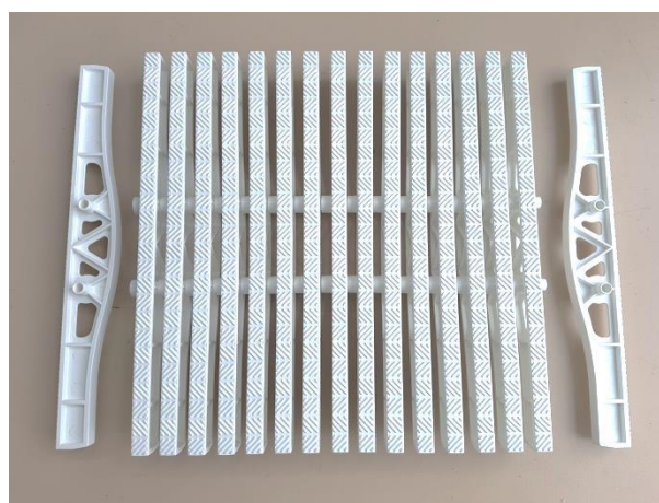
FIG. 1 'PERPENDICULAR' POOL GRATE COMPONENTS AS DELIVERED
